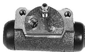
10411212 TOYOTA FD15 LH W/O NIPPLE 7/8" (M10x1.25) TO-716-1
