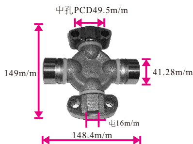
TCM FD180 KOMATSU FD85(3型) 49.5x148.4x16m/m Φ14x41.28(圓) 378(AE7999)
