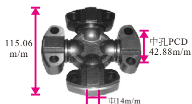
131-10-46110 308-20-21010 KOMATSU FD50/60/80 YALE FD50/60 DAEWOO FD70 42.88x115.06m/m 川崎65鏟土機 C5-5177X (GUKO-5C)
