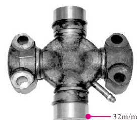
37101-33900-71 TOYOTA 5/6FD60/70 32x83.9x115 m/m GU-555
