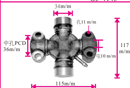
37201-30510-71 TOYOTA 6/7FD40 MITSUBISHI S4S FD30 (紫) / S6S 34x115x117 m/m G5-5015X-1
