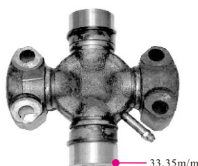
37112-33900-71 TOYOTA 5FD60 33.35x115.6x118 m/m GU-554(G5-5015X)
