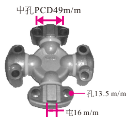
TCM FD250 KOMATSU SHOVELLER (鏟土機) 49.2x148.4x16m/m Φ14m/m G5-7126
