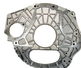
32111-23371-71 TOYOTA 7FD25 (2Z) CASE (鋁件)
