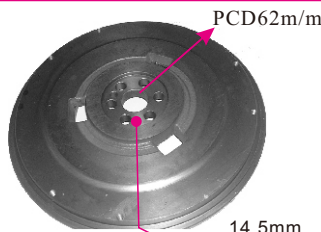
113T 7孔 12310-10H01 NISSAN (TD27) Φ35*316m/m DK-3016
