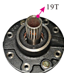
15583-80221 TCM 3T Z-5/T6 CHARGING PUMP 19T(粗牙) UJ-5047-1
