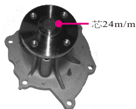
16100-78700/1-71 TOYOTA 7/8FD25 (2Z) PW18-83
