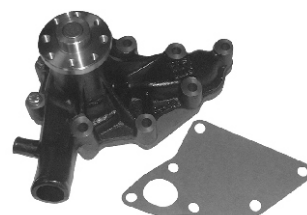
5-13610-047-Z 9-13610-394-Z TCM C240FD15-30 (MADE IN JAPAN) WPT-503
