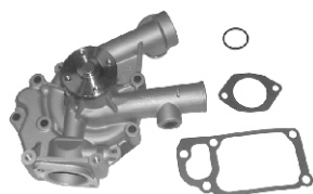
16100-78300-71 TOYOTA 5/6FD25/40 (1Z) (MADE IN JAPAN) WPT-501 WPT-501-1
